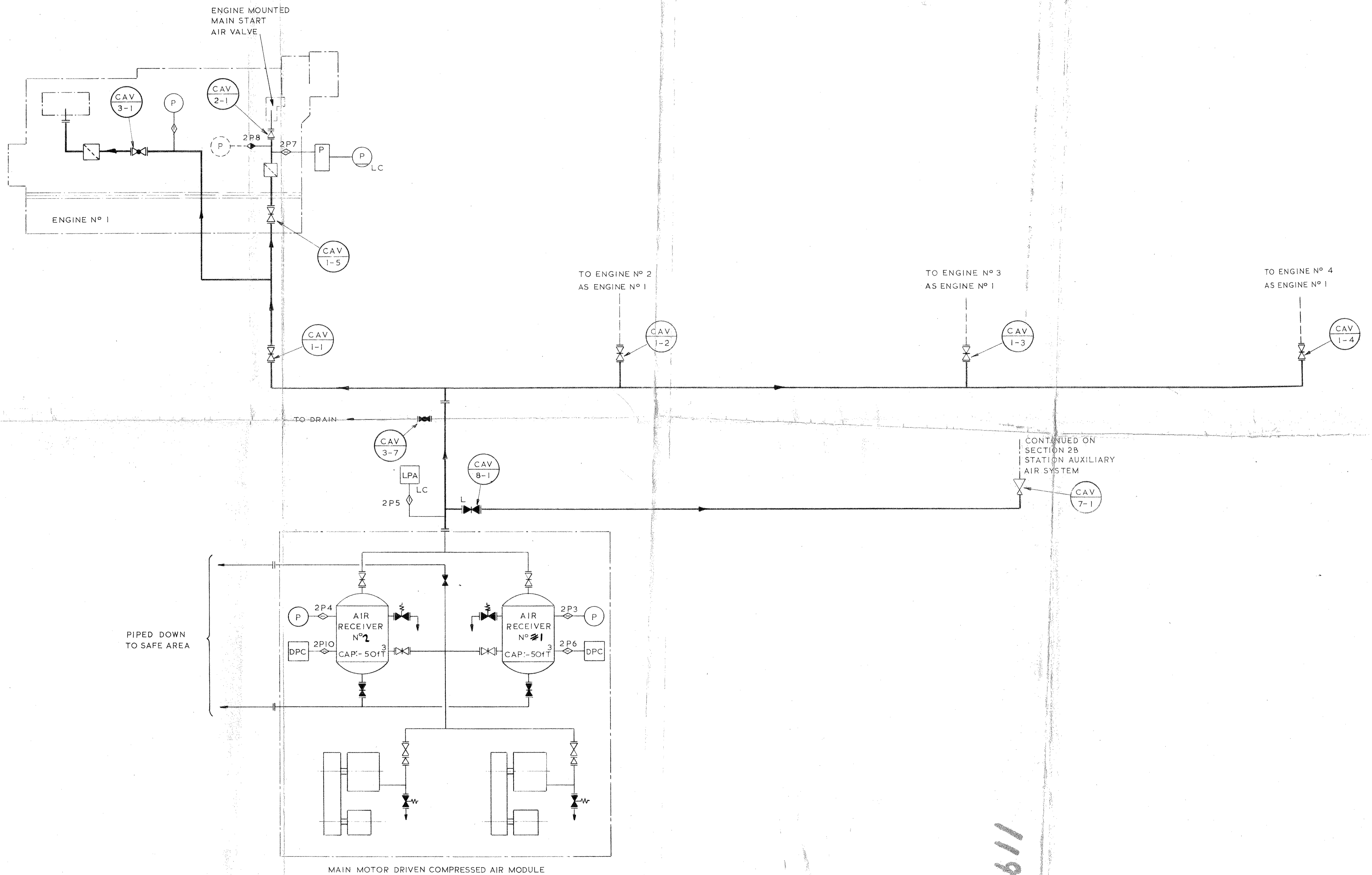
SECTION 2A - ENGINE START AIR SYSTEM
